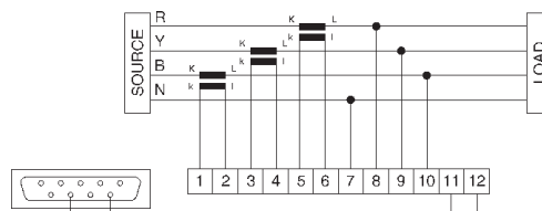
3 Phase 3 Element 4 Wire
